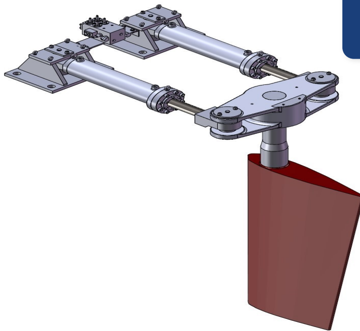
SS/SP Series Electro-Hydraulic Steering Gear System
