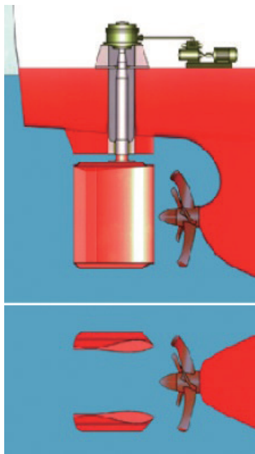
Outline of VecTwin Rudder
